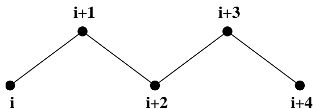
Figure 4.18: Atoms along an alkane chain.
