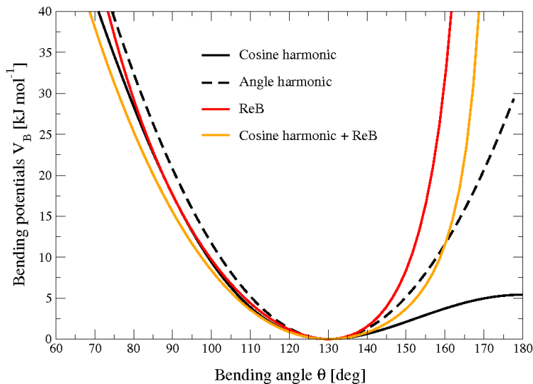
Figure 4.8: Bending angle potentials: cosine harmonic (solid black line), angle harmonic (dashed black line) and restricted bending (red) with the same bending constant k_\theta = 85 \text{ kJ mol}^{-1} and equilibrium angle \theta_0 = 130^\circ . The orange line represents the sum of a cosine harmonic ( k = 50 \text{ kJ mol}^{-1} ) with a restricted bending ( k = 25 \text{ kJ mol}^{-1} ) potential, both with \theta_0 = 130^\circ .
